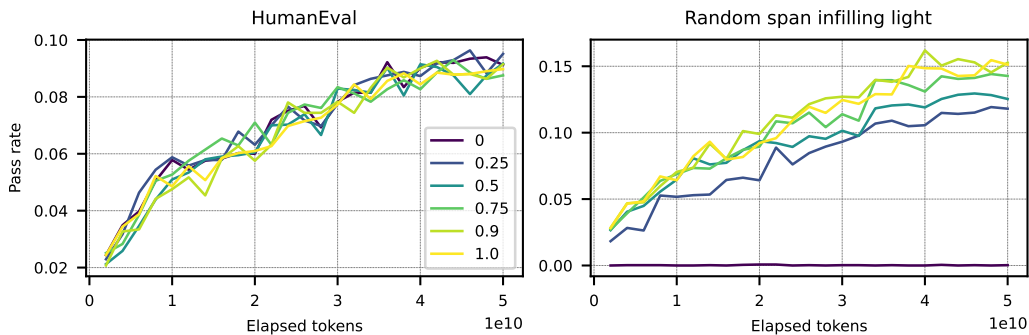
Figure 5: In-run evaluation of coding benchmarks with temperature 0.8 and 25 samples per task. Using higher FIM rates do not have a noticeable effect on HumanEval performance. A higher FIM rate shows stronger infilling capabilities on the light random span infilling benchmark.
